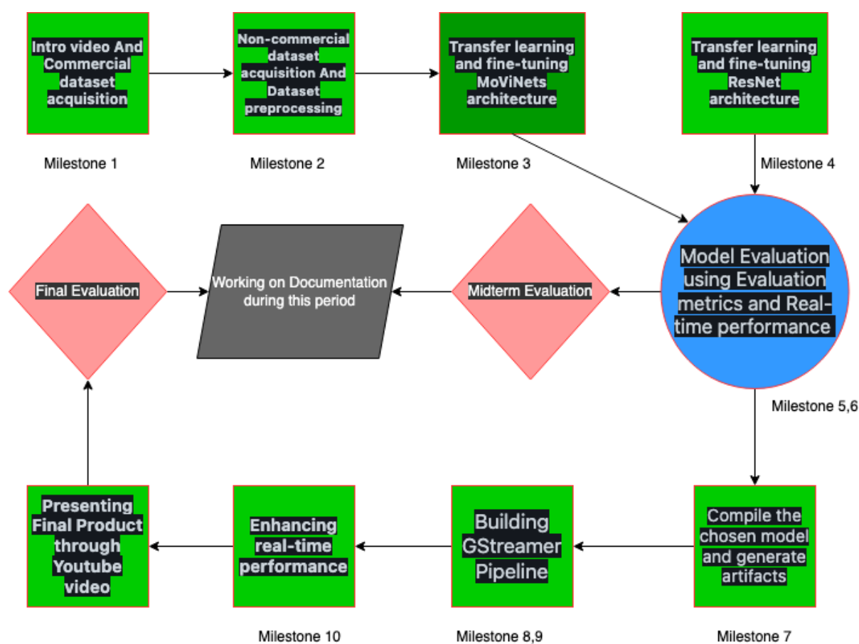
Figure 6: Project Workflow
